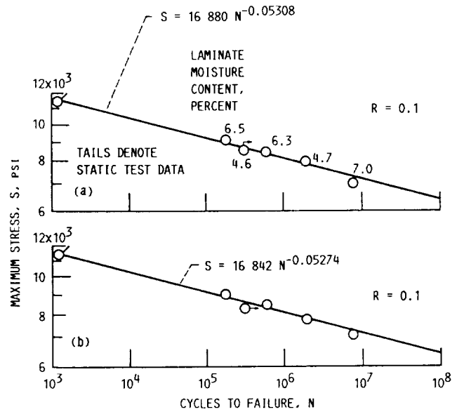
(a) Data not corrected for moisture content. Correlation coefficient, r , -0.9891 . (b) Data corrected to 6 percent laminate moisture content ( K = 1.21 ). Correlation coefficient, r , -0.9930 .
