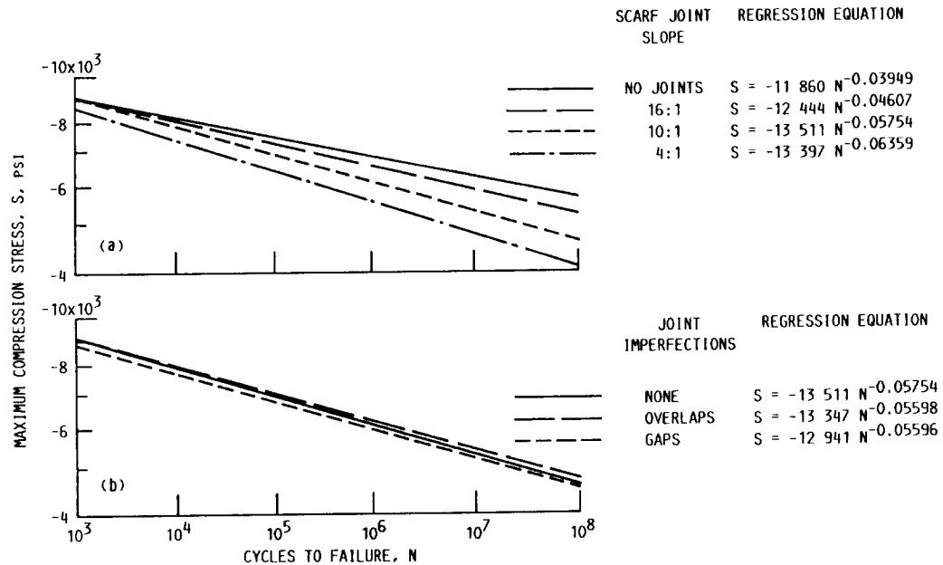
(a) Summary of effects of scarf slope. (b) Summary of effects of imperfections in 10:1-slope scarf joints.
