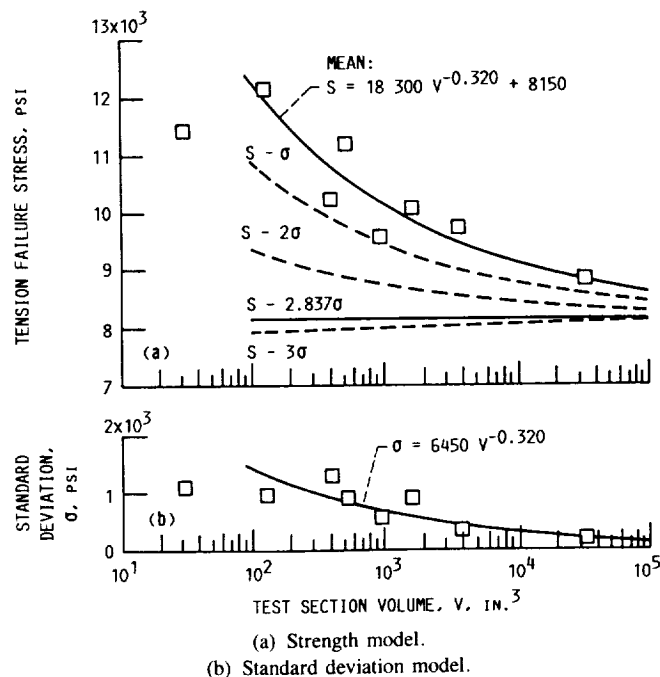
Figure 3.—Strength and standard deviation models for static tension in laminated Douglas fir/epoxy specimens with scarf joints in laminations. Data corrected to 6 percent laminate moisture content ( K = 1.21 ). Veneer grade, A+.
