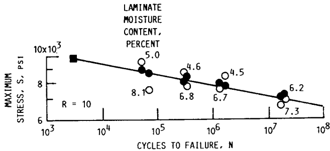
Figure 1.—Moisture correction of data for compression fatigue ( R = 10 ) parallel to grain in laminated Douglas fir/epoxy specimens. Veneer grade, A+. Data from figure 4.2-1 of chapter IV.
