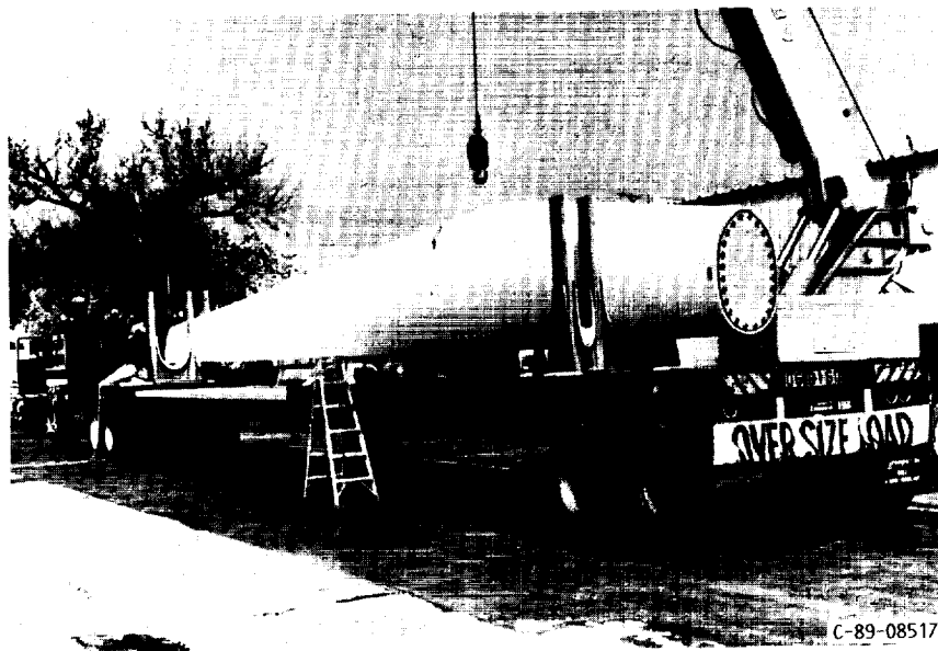
Figure 12.—Laminated fir/epoxy blade for 142-ft-diameter Westinghouse 600-kW commercial wind turbine.
