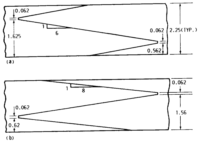
(a) 1:6 Slope. Pitch, 2.125 in. (b) 1:8 Slope. Pitch, 1.625 in.
