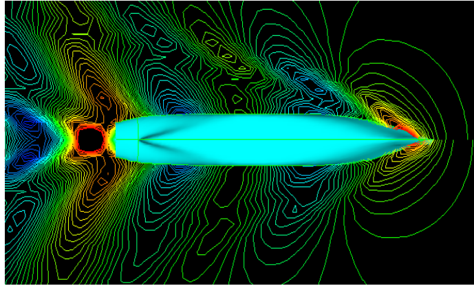
Representation of the contours of wave height
