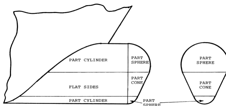
Bulb built from simplified conic shapes (Lamb, 1986 )
