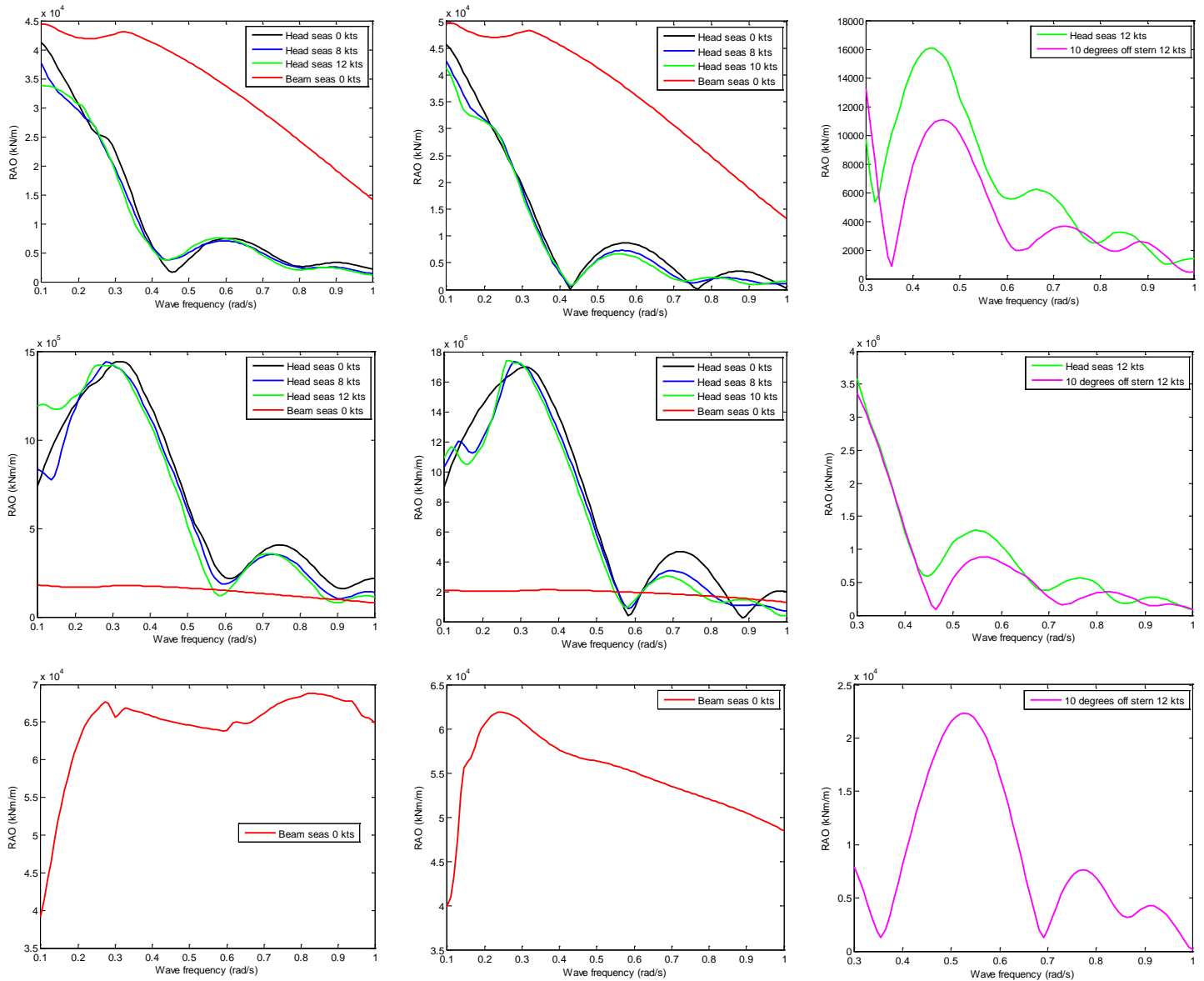
Figure 17: Wave-induced heave force (top), pitch moment (middle) and roll moment (bottom) of Ship F (left), Ship G (middle) and Ship D (right) as calculated using OCTOPUS
