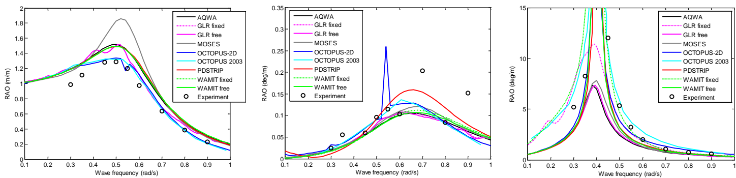
Figure 12: Heave (left), pitch (middle) and roll (right) of Ship F in beam waves at zero forward speed
