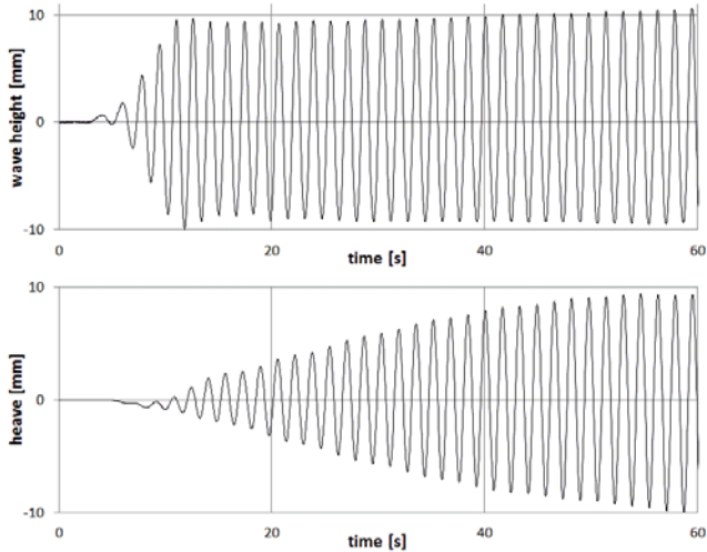
Figure 13: Scale 1:50 measured heave motion for Ship F in head seas at zero speed, full-scale wave frequency 0.55 rad/s.
