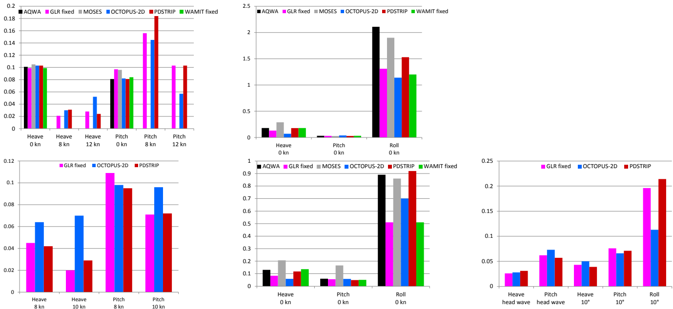
Figure 18: Differences between numerical and experimental results, plotted from Table 4. Top left: Ship F, head seas; top middle: Ship F, beam seas; bottom left: Ship G, head seas; bottom middle: Ship G, beam seas; bottom right: Ship D
