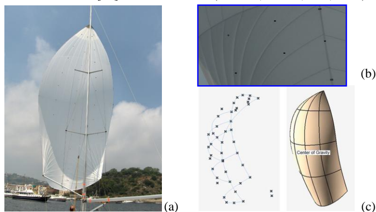
Fig. 7. (a) marker acquisition; (b) marker on the sail; (c) 3D NURBS surfaces.
