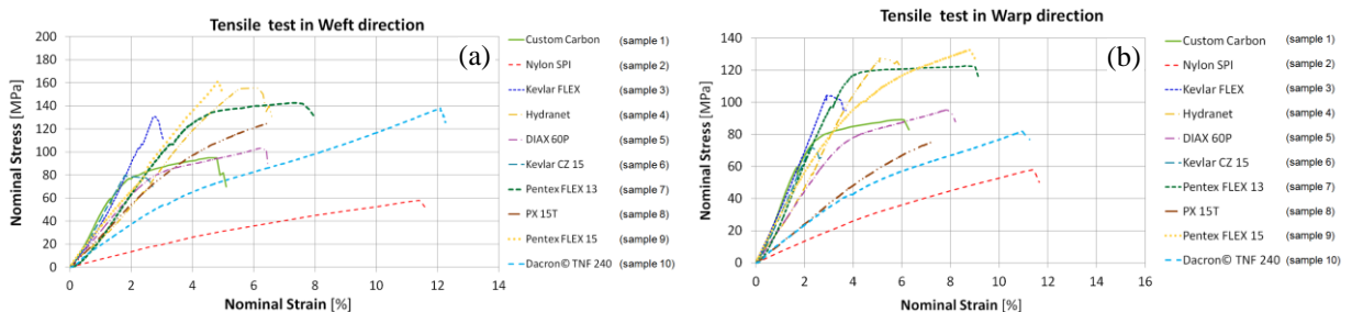
Fig. 3. Nominal Stress-Nominal Strain curves in: (a) weft direction; (b) warp direction.
