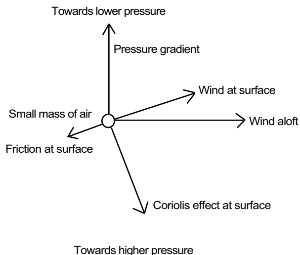
Fig. 2 (b) Forces on a particle of air in the influence of friction.
