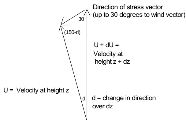
Fig 4: The relationship between stress and wind velocity vectors.
