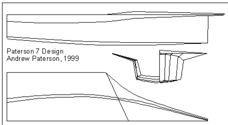
Like the Slug, the Paterson 7 has the waterplane further aft than its predecessor. The shape of the boat is characteristic Patterson, with very vertical topsides, and the flare is particularly flat.
