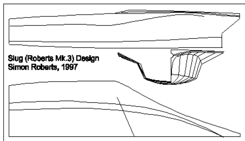
The first true 1997 rules design, the Slug features a distinctively “wavy” flare line, and waterplane rather further aft than its rule-constrained predecessors.
