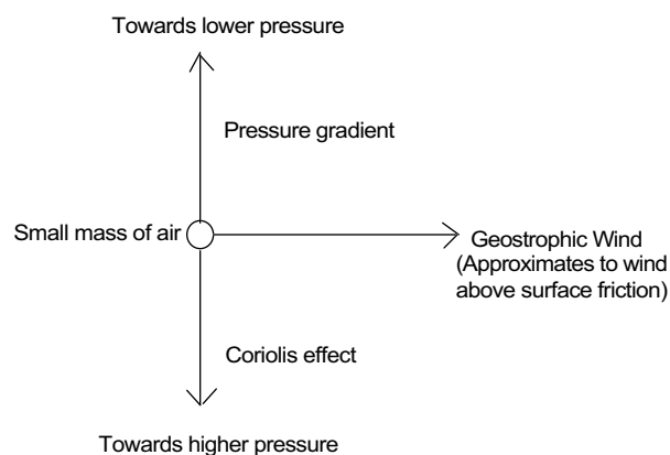
Fig. 2 (a) Forces on a particle of air in the free atmosphere.
