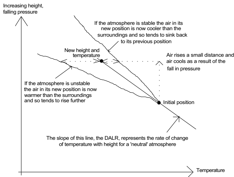
Fig 1: Neutral, stable and unstable temperature profiles.
