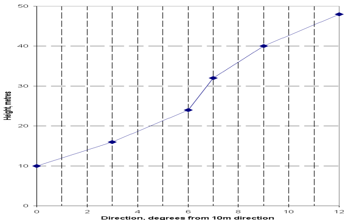
Fig. 5 Changes in wind direction with height measured at Sellafeld at 1200UTC on the 9th April 1997. Directions are 10-minute averages.
