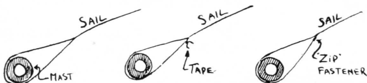
FIG. 1. Sections of Pocket Luff Sails.
