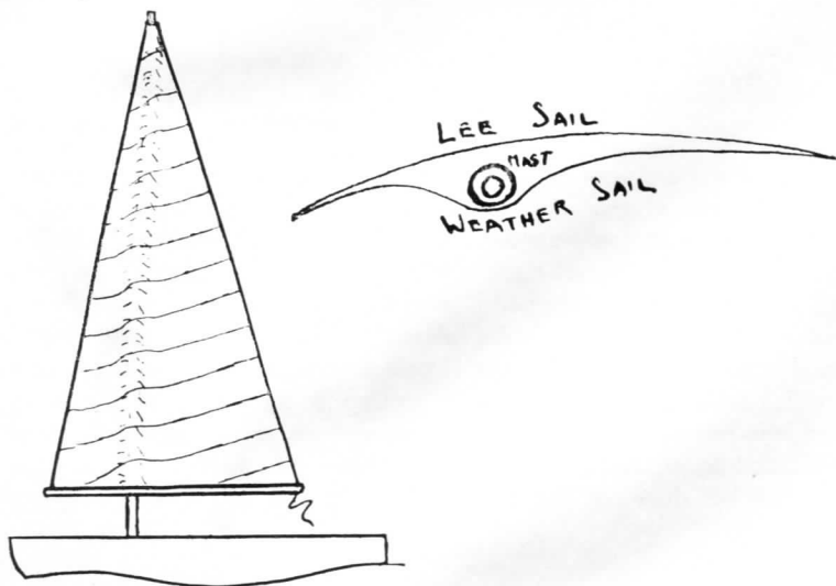
FIG. 7. A Double Lugsail.
