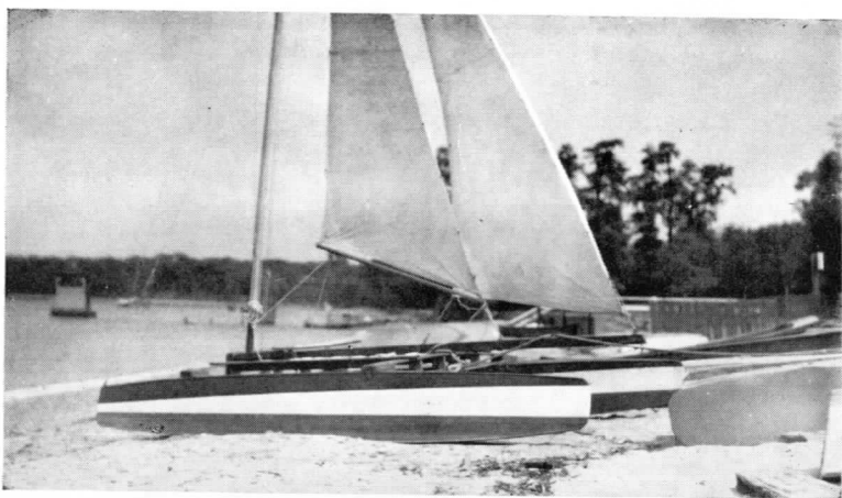
Victor Tchetchet's Mastaft Rig.
