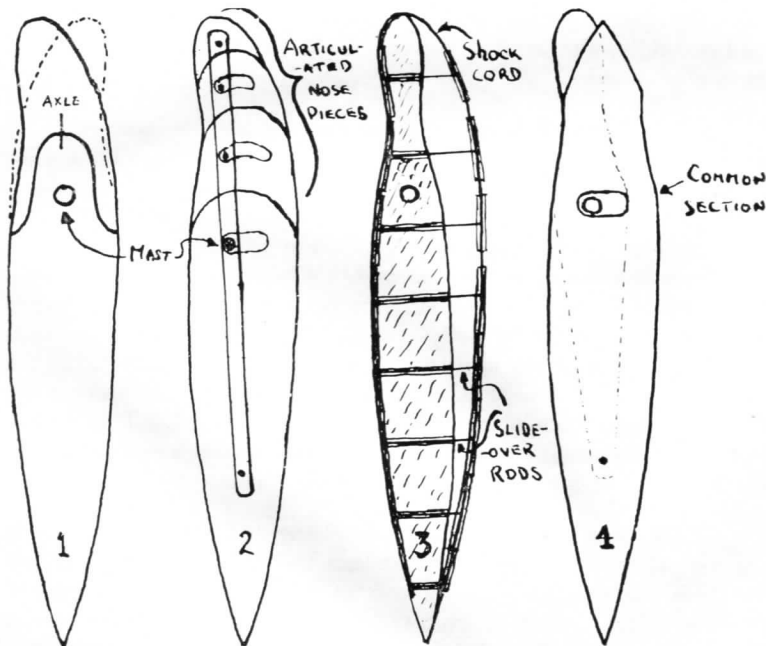
FIG. 9. Four types of Asymmetrical Formers.
