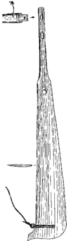
A Viking Age Rudder, showing it's slender cross-section and the various anchor points, trailing line to raise it and the point where the tiller bar was slotted in.
