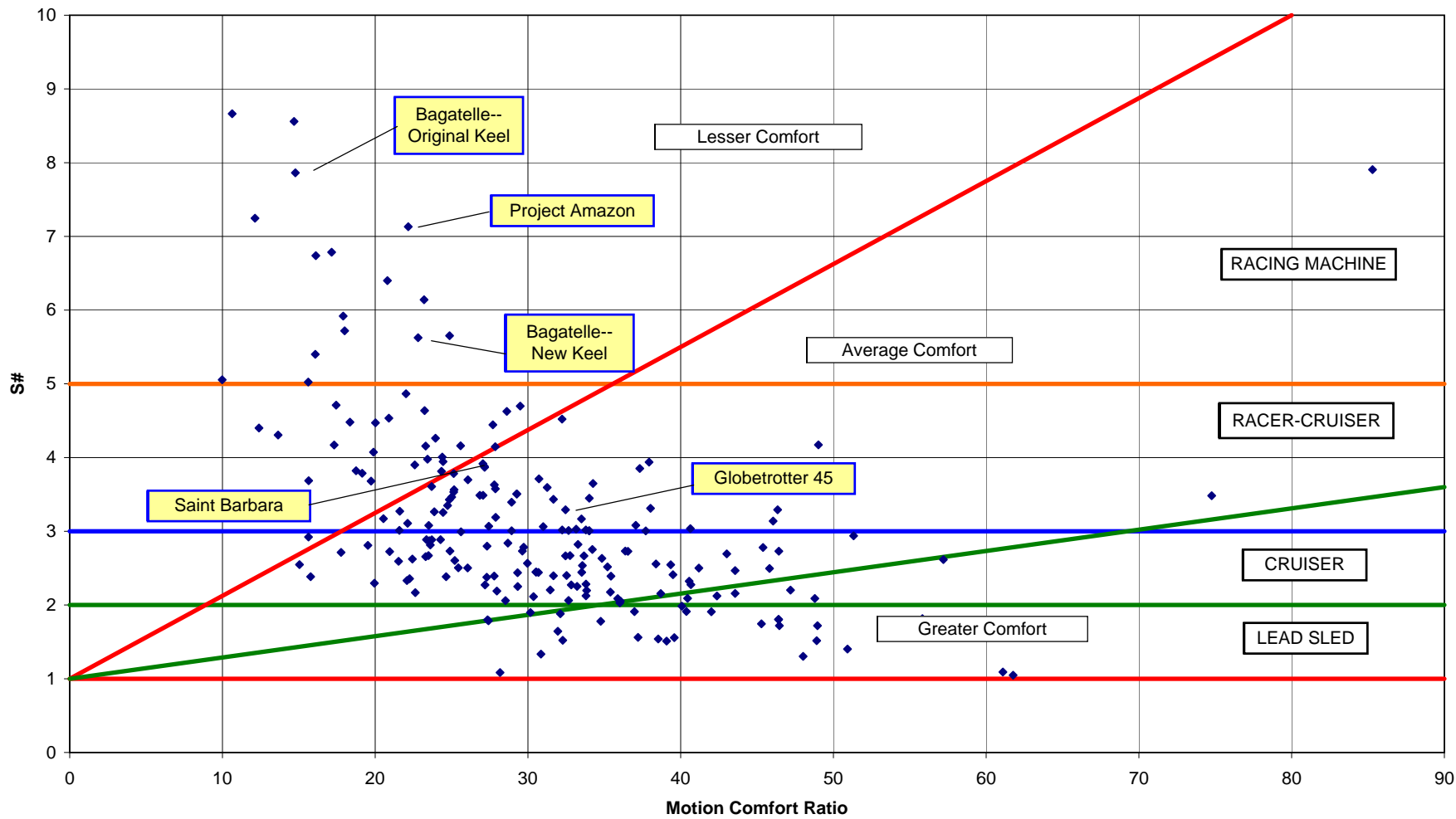
MCR Chart 02--S# vs MOTION COMFORT RATIO
