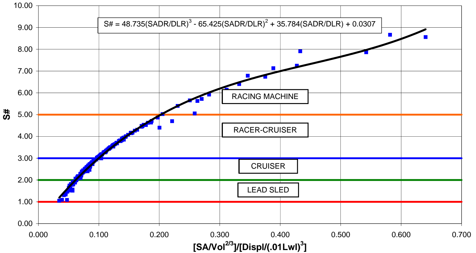
S# CHART 03 -- S# v. [SA/Vol^{2/3}]/[D/(.01Lwl)^3]
