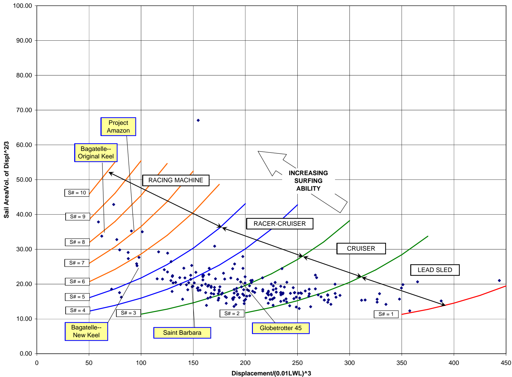
S# CHART 02 -- Sail Area/Displ vs. Displ/Length
