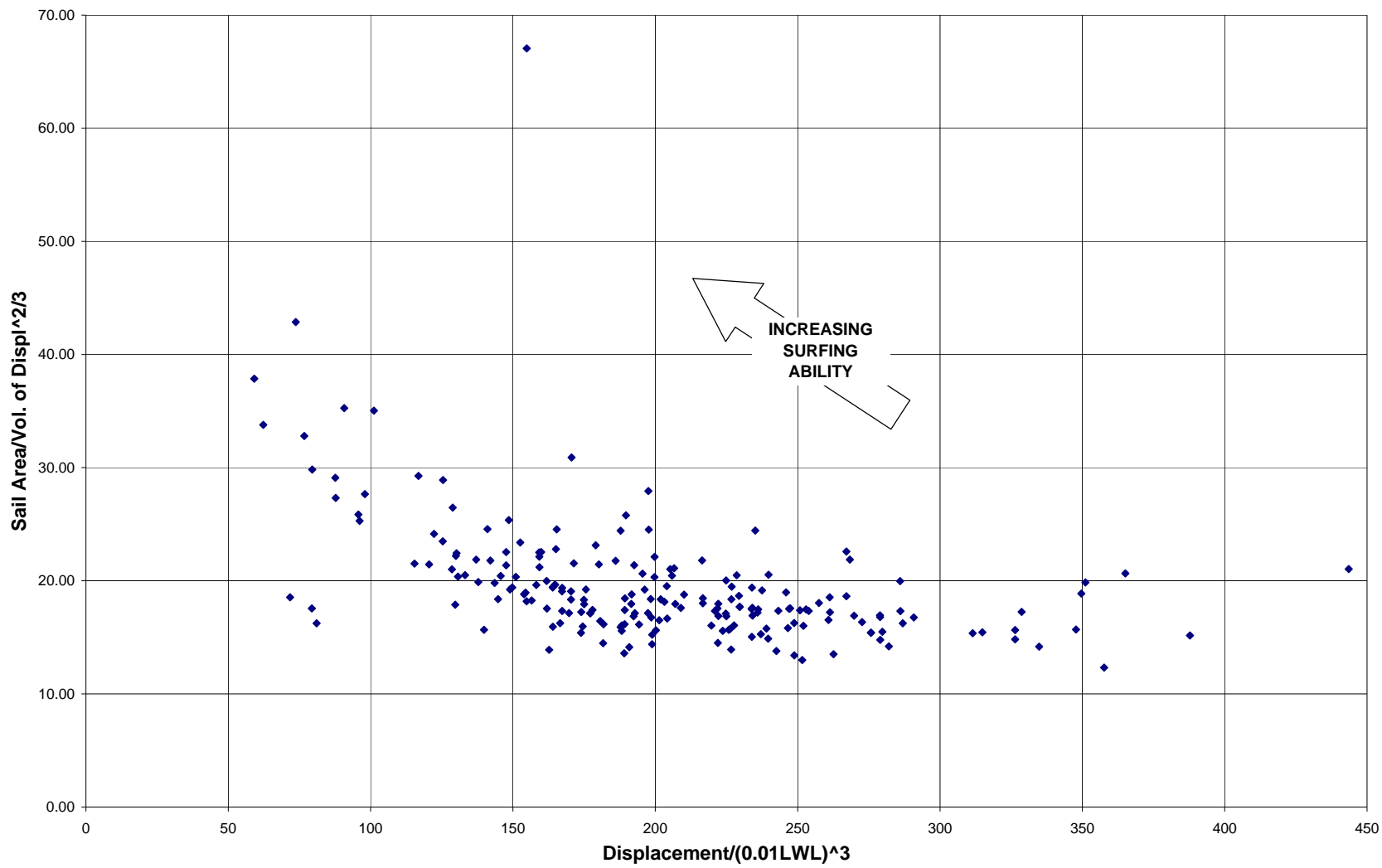
S# CHART 01 -- Sail Area/Displ vs. Displ/Length
