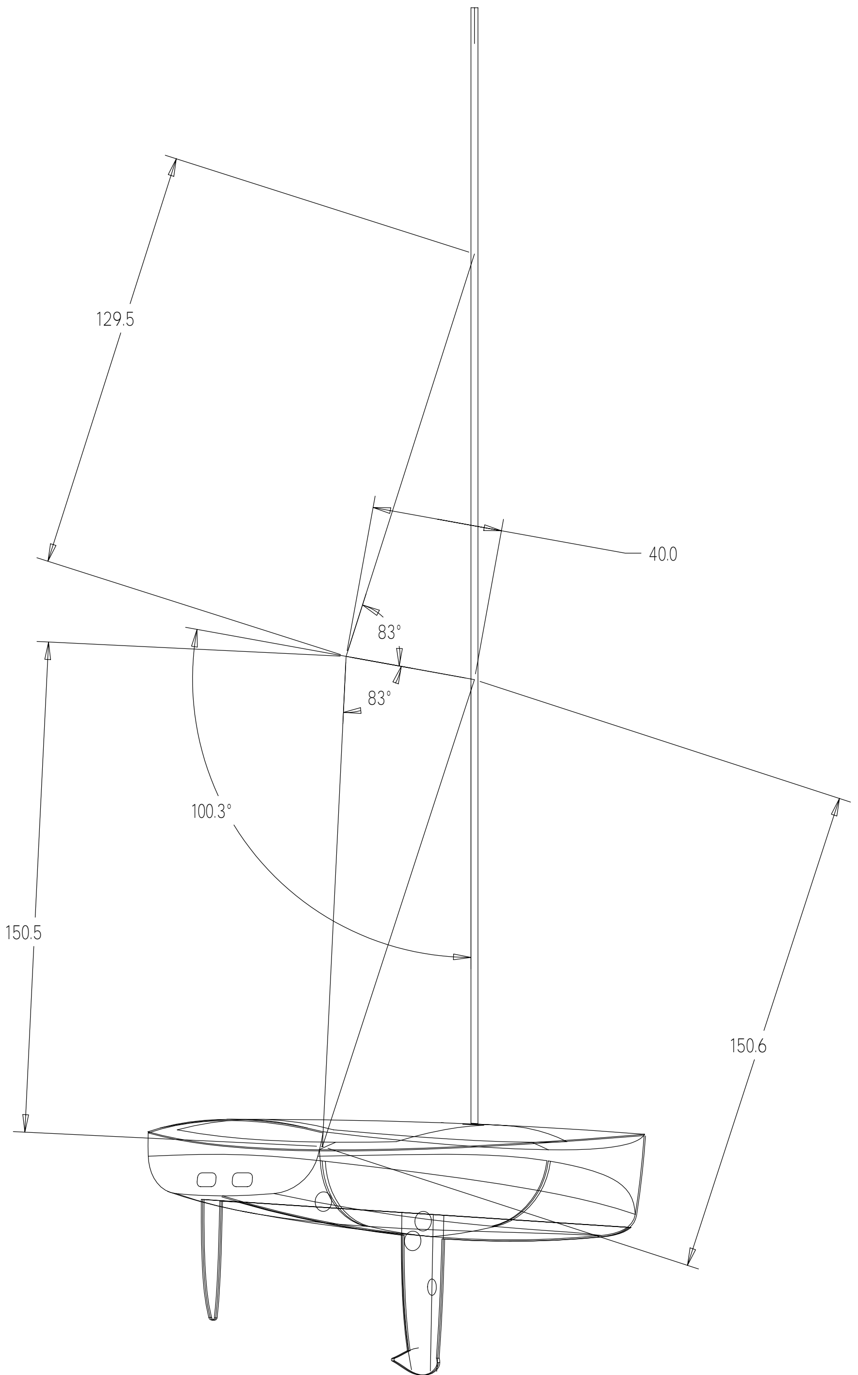
TRUE VIEW OF SHROUD SHOWING ACTUAL WIRE LENGTHS TO DECK ADD ALLOWANCES FOR LOWER TURNBUCKLE
