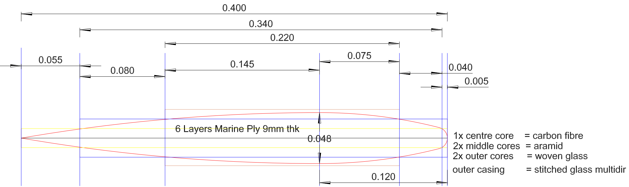
Centre Board Naca 63-012
